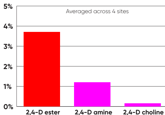
Chart 1. Cumulative 2,4-D Vapor Loss at 70 Hours After Treatment
